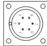
CN1 REMOTE CONNECTOR
